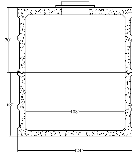
End Section
