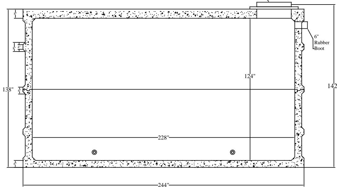
Side Section
